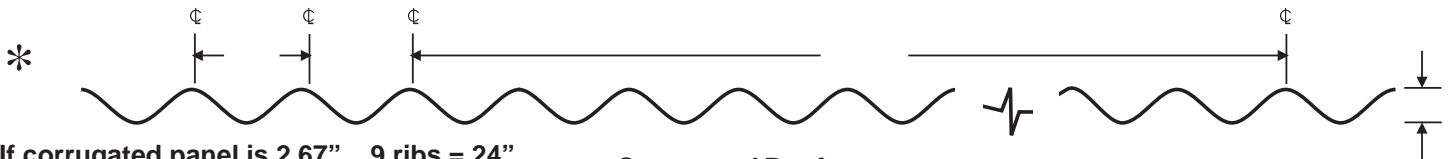
Corrugated Roof
